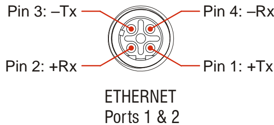
Figure T1.8 M12 Ethernet Connector Pinout
