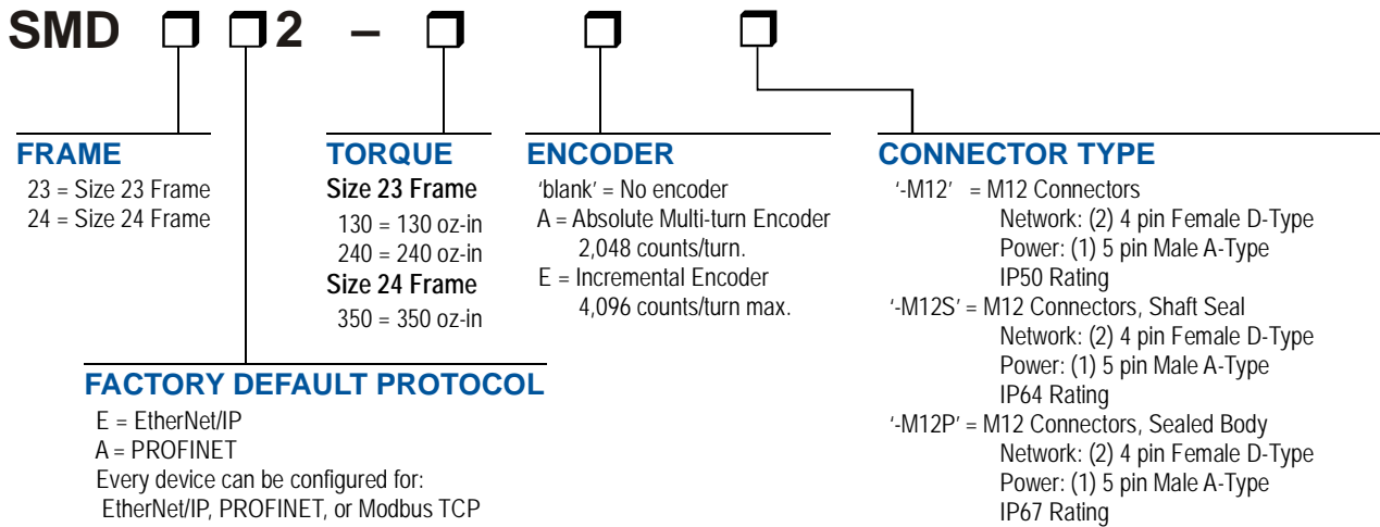
Figure R1.2 Part Numbering System
