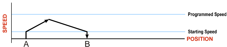
Figure R2.5 A Triangular Profile
