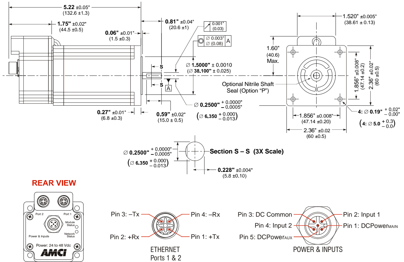
Figure T1.2 SMD24E2 Outline Drawing
