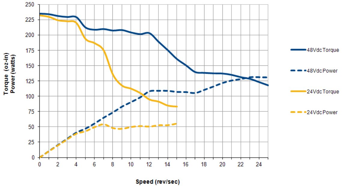
Figure R1.8 SMD23E2-240 Torque and Power Curves
