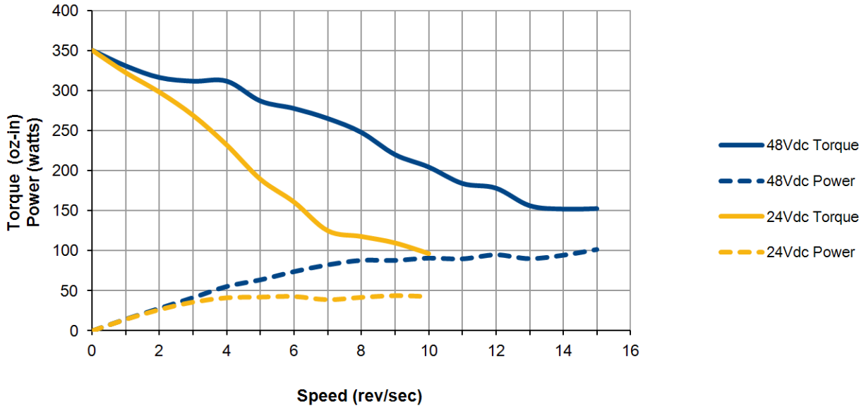
Figure R1.9 SMD24E2-350 Torque and Power Curves
