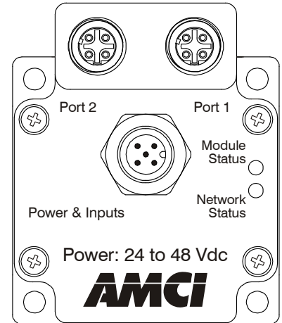
Figure R1.4 Connector Locations
