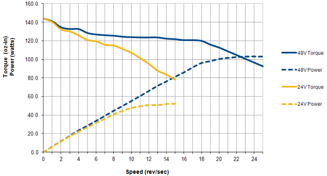
Figure R1.7 SMD23E2-130 Torque and Power Curves
