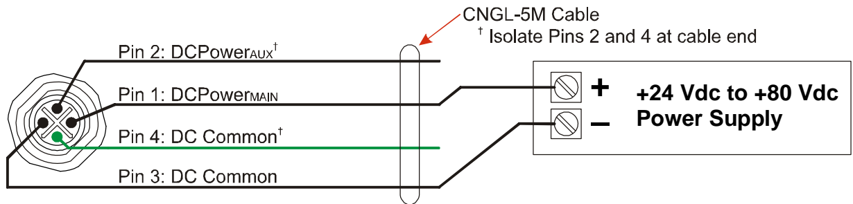
Figure T1.3 SMD34E2 Main Power Wiring
