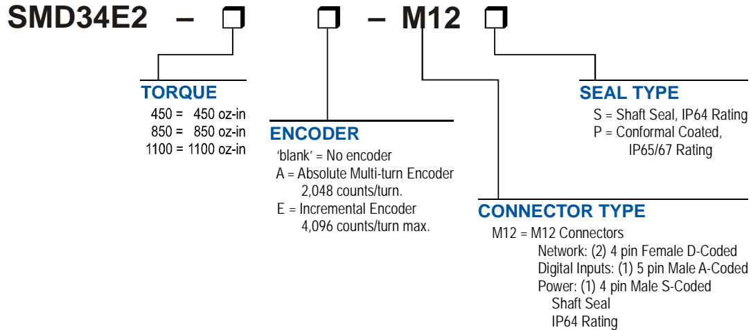
Figure R1.2 Part Numbering System
