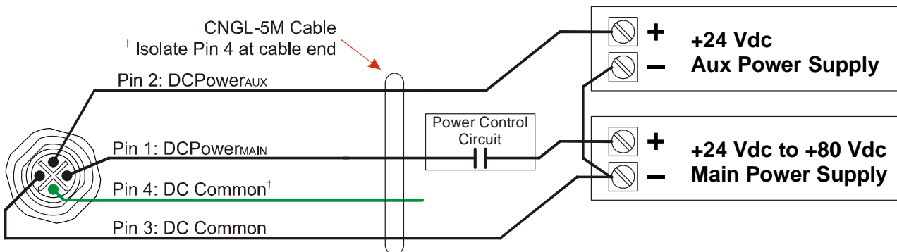
Figure T1.5 SMD34E2 Auxiliary Power Wiring, Single Supply
