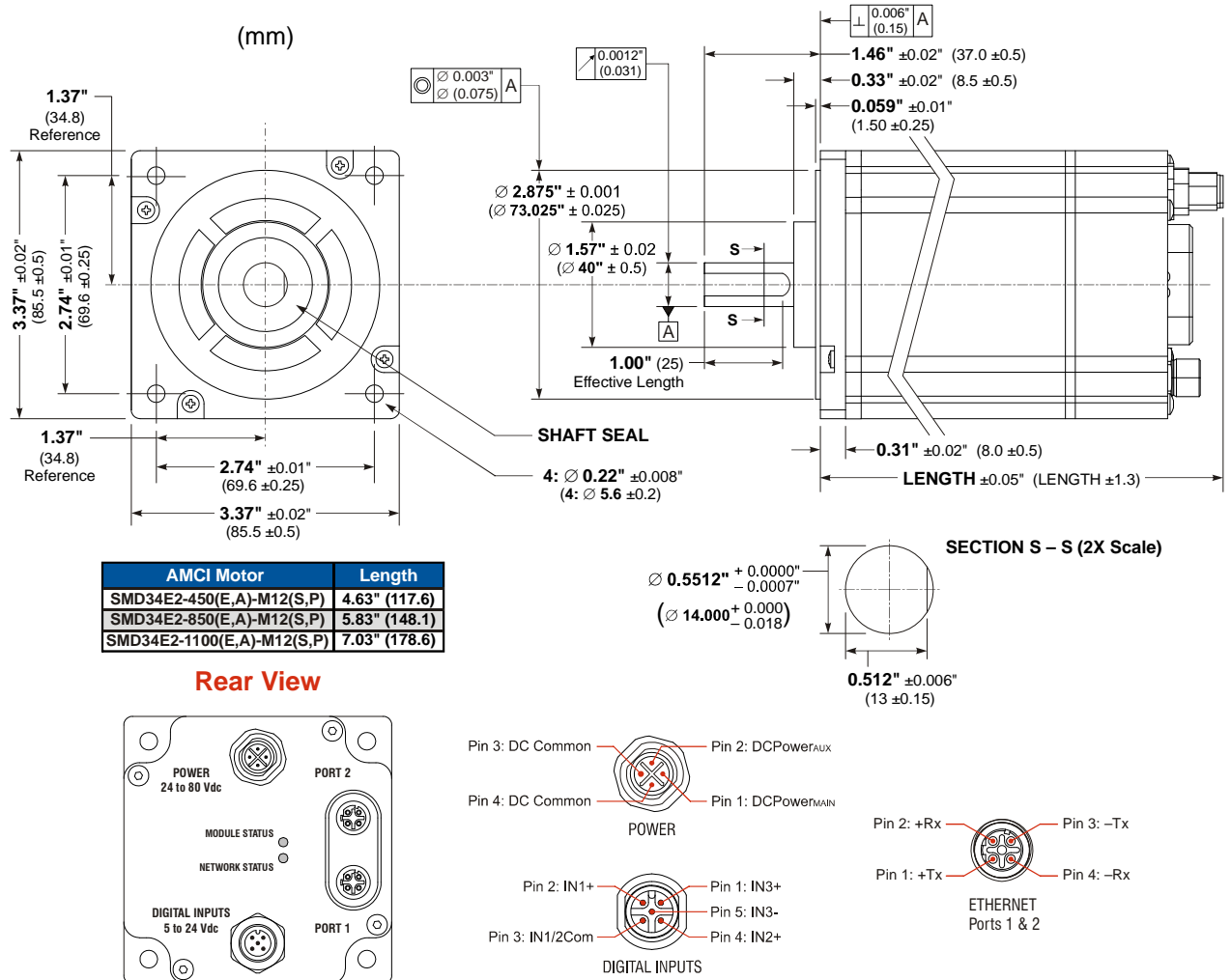
Figure T1.1 SMD34E2 Outline Drawing
