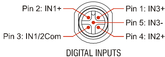
Figure R1.6 M12 Input Connector
