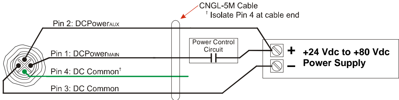
Figure T1.4 SMD34E2 Auxiliary Power Wiring, Single Supply
