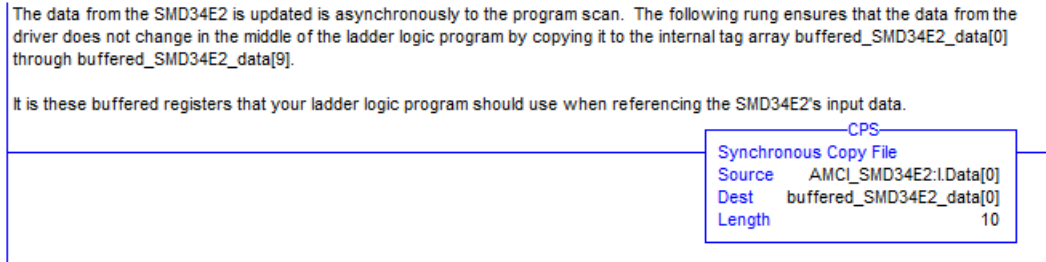
Figure T4.4 Buffer I/O Data
