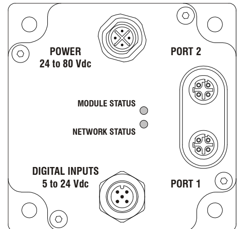
Figure R1.4 SMD34E2 Connector Locations
