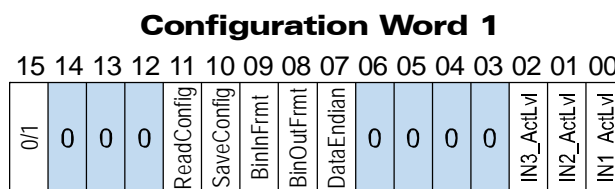
Figure R5.2 Configuration Mode: Config Word Format
