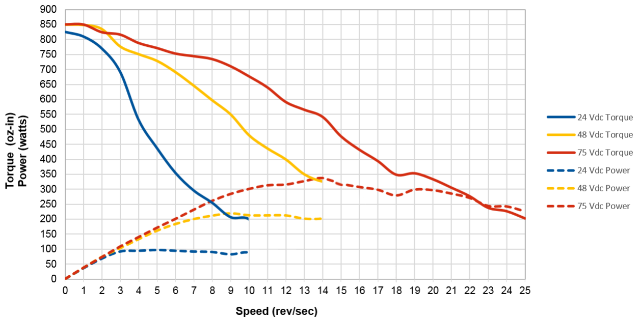
Figure R1.9 SMD34E-850 Torque and Power Curves
