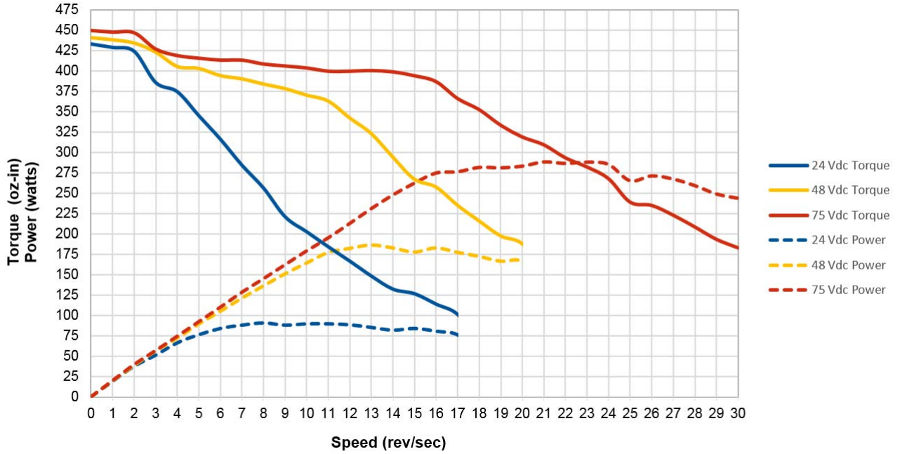
Figure R1.8 SMD34E-450 Torque and Power Curves
